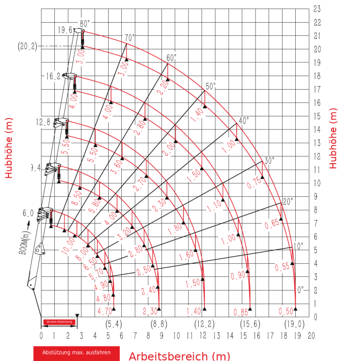
Lastdiagramm (t)
